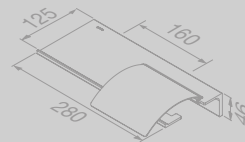
Planchet 28 cm met toilethouder met klep (Black) Bathroom shelf 28 cm with toilet roll holder with cover (Black)
