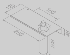
Planchet 28 cm en zeepdispenser 200 ml met handdoekhaak (Black/Brushed stainless steel) Bathroom shelf 28 cm with towel hook and soap dispenser 200 ml (Black/Brushed stainless steel)
