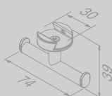
Handdoekhaak (Brushed stainless steel) Towel hook (Brushed stainless steel)
