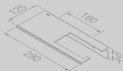
Planchet 28 cm met toilethouder zonder klep (Black) Bathroom shelf 28 cm with toilet roll holder without cover (Black)
