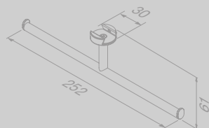
Toiletrolhouder zonder klep dubbel (Brushed stainless steel) Toilet roll holder without cover double (Brushed stainless steel)
