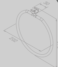
Handdoekring (Brushed stainless steel) Towel ring (Brushed stainless steel)
