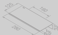
Planchet 28 cm met toilethouder zonder klep dubbel (Black/Chrome) Bathroom shelf 28 cm with toilet roll holder without cover double (Black/Chrome)
