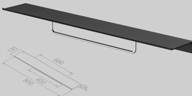
Planchet 80 cm met handdoekrek 40 cm (Black/Brushed stainless steel) Bathroom shelf 80 cm with towel rail 40 cm (Black/Brushed stainless steel)
