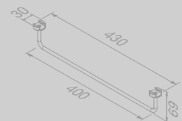
Handdoekrek 40 cm (Brushed stainless steel) Towel rail 40 cm (Brushed stainless steel)
