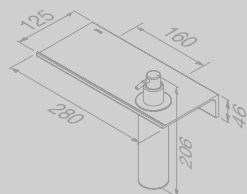
Planchet 28 cm met handdoekhaak en zeepdispenser 200 ml (Black) Bathroom shelf 28 cm with towel hook and soap dispenser 200 ml (Black)
