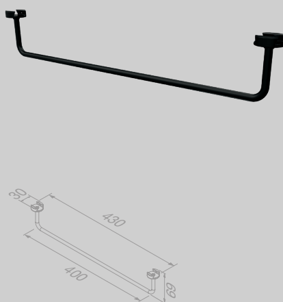
Handdoekrek 40 cm (Black) Towel rail 40 cm (Black) 918207-06
